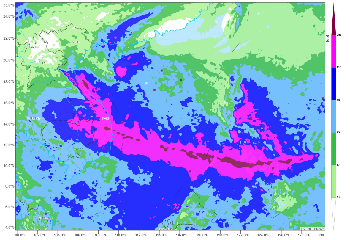
Figure 2 Forecasted Accumulated Precipitation from 08:00 on November 3 to 08:00 on November 8 (BJT) (Unit: mm)
