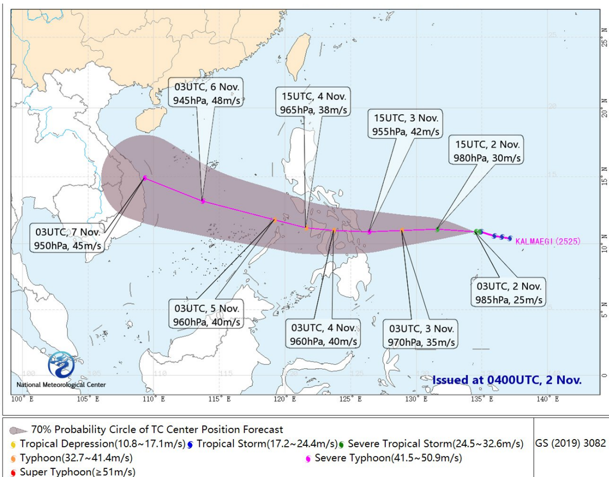
Figure 1 120 Hour Probabilistic Track Forecast for Typhoon "KALMAEGI"
